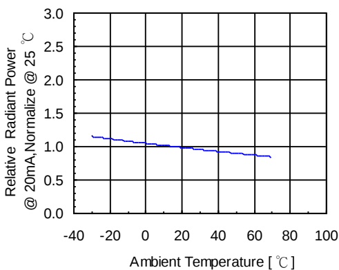
Fig 6. Relative Radiant Power vs. Temperature
