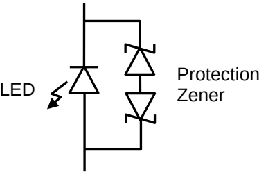
Equivalent Circuit
